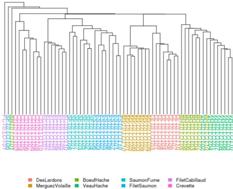
single linkage clustering tree
