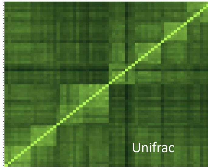
Heatmap plot of the beta distance : unifracs
