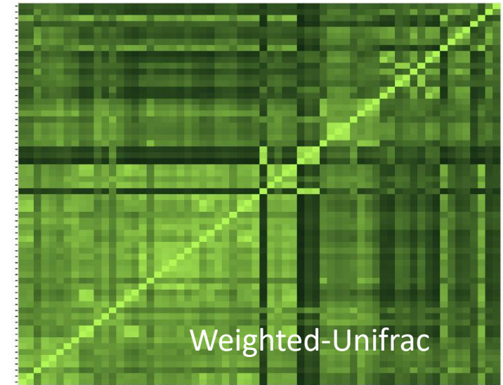
Heatmap plot of the beta distance : wunifracs
