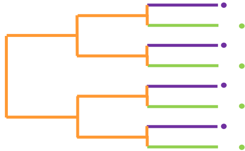
Low Unifrac / High Jaccard
