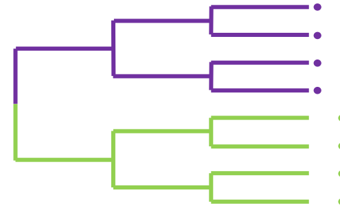
High Unifrac / High Jaccard
