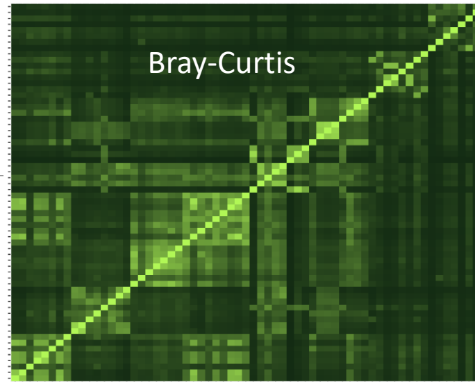
Heatmap plot of the beta distance : bray
