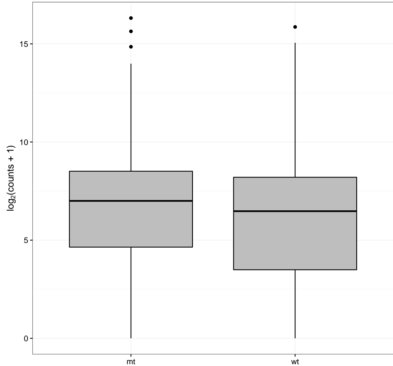
Boxplot on raw pseudo-counts
