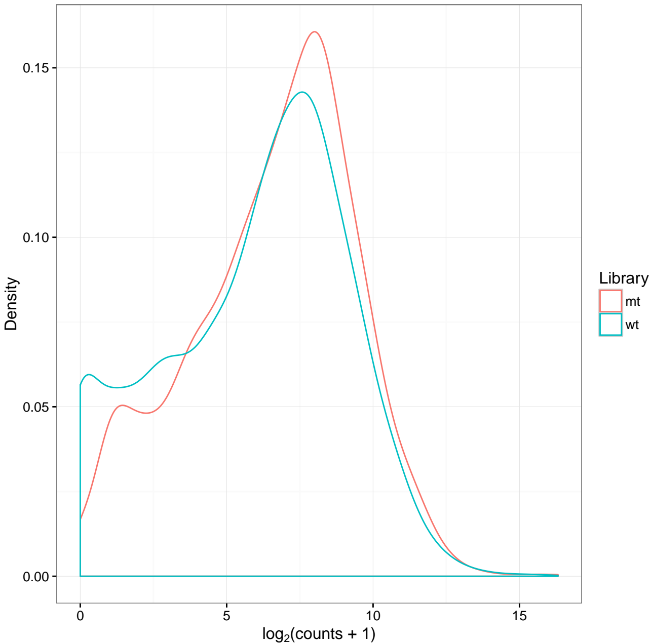
Density plot on raw pseudo-counts
